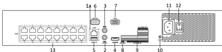
DS-7732NI-I4/16P
